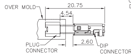
MATING CONDITION
