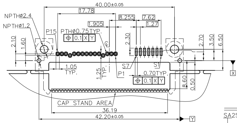
TOP VIEW RECOMMENDED PCB LAYOUT TOLERANCE: +/-0.05mm
