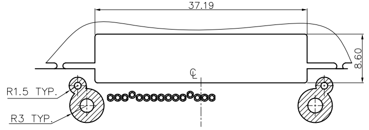
BOTTOM VIEW RECOMMENDED PCB LAYOUT TOLERANCE: +/-0.05mm
